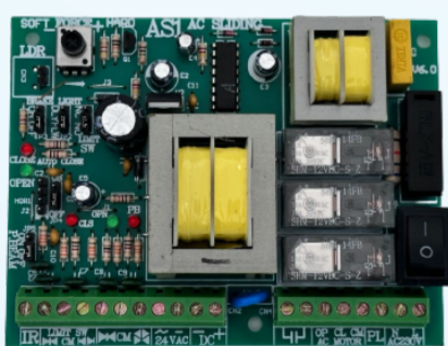
AS1 Sliding Type Control Panel
